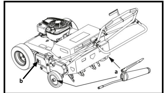
FIGURE 2: a) Grease fittings b) Locations of idler sprocket for chain tension. Other location is the opposite side of the machine
