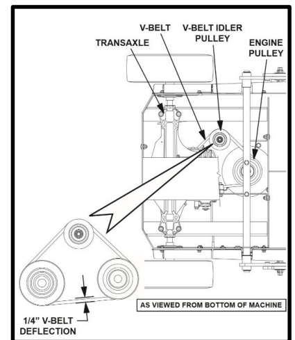
FIGURE 3: V-Belt Pulley location and tension check
