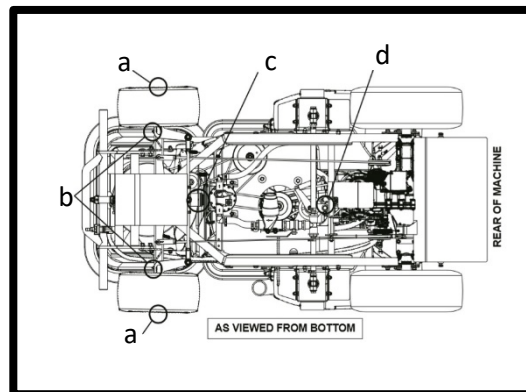
FIGURE 1: a) 2 Front Wheel Bearings, b) 2 Front Wheel Spindles, c) 1 Front Axle, d) Idler Arm
